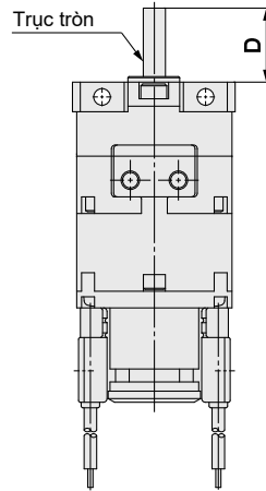
2 Trục/CDRBU2JU
