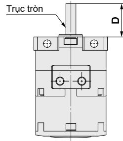
2 Trục/CRBU2JU
